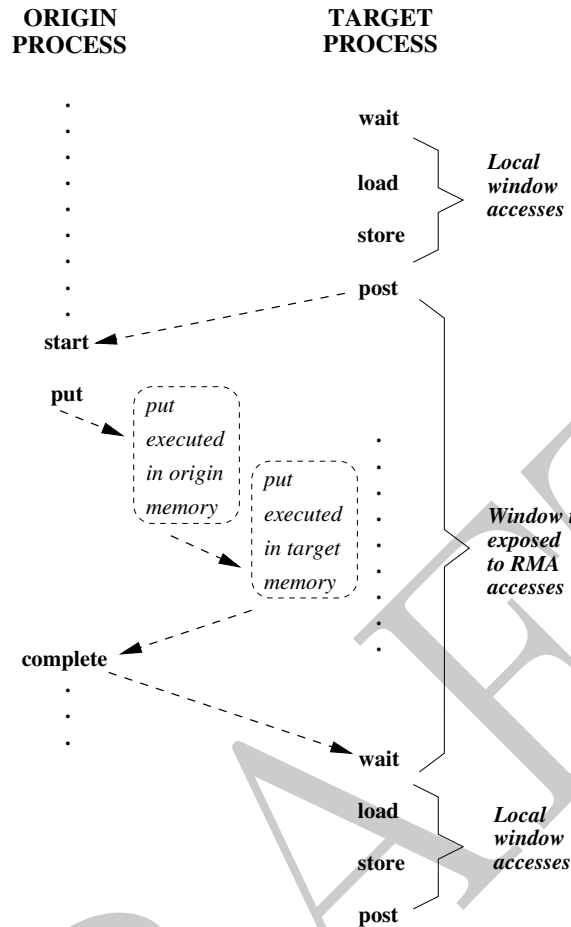
Figure 11.2: Active target communication. Dashed arrows represent synchronizations (ordering of events).
