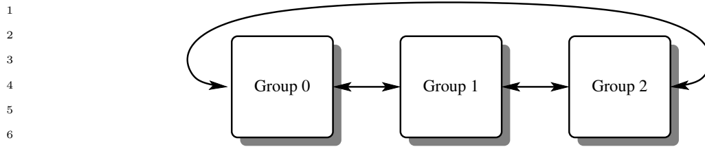
Figure 6.5: Three-group ring
