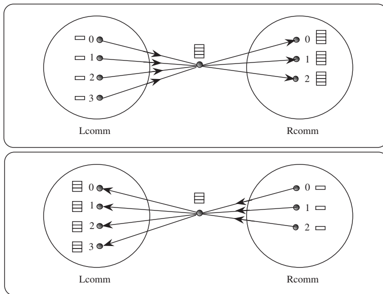
29 Figure 5.2: Intercommunicator allgather. The focus of data to one process is represented, 30 not mandated by the semantics. The two phases do allgathers in both directions.
