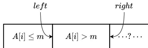
Figure 1: All A[i] \leq m where 0 \leq i < left ; while A[i] > m where left \leq i < right . The rest are yet to be scanned.
