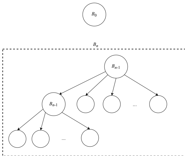
Figure 10.1: Binomial tree
