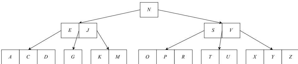
Figure 7.10: Before delete
