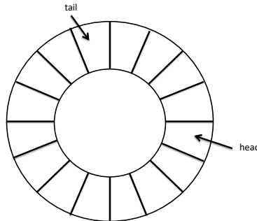
Figure 11.3: Circular buffer.
