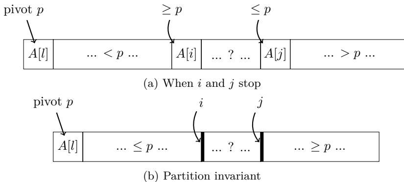
Figure 13.3: 2-way scan
