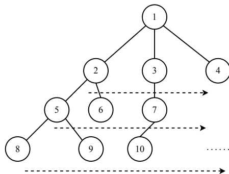
Figure 15.10: Start from 1, check all options 2, 3, 4 for the next step; then all option for the 3rd step, ...
