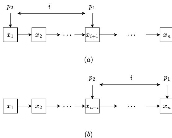
Figure 1.2: Sliding window. (a) p_2 starts from the head, behind p_1 in i steps; (b) When p_1 reaches the tail, p_2 points to the i -th element from right.
