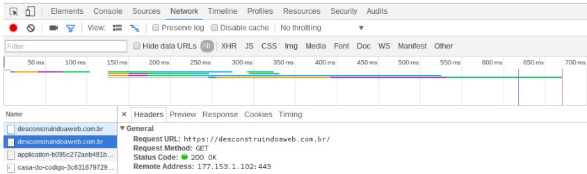
Figura 4.1: O método GET no developer tools do Chromium
